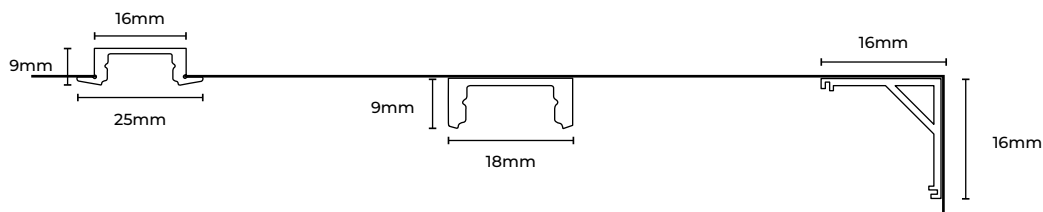
Recessed
